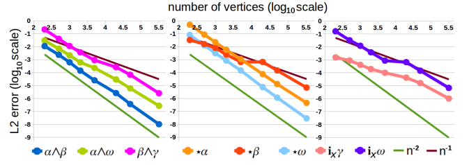
Figure 2: L^2 errors of approximation of the wedge product ( L ), Hodge star ( C ), and contraction ( R ) on a set of irregular polygonal meshes on torus. Here \alpha = x^2 + y^2 , \beta = -ydx + xdy , \gamma = -2xzdx - 2yzdy + 2(x^2 + y^2 - \sqrt{x^2 + y^2})dz , \omega = \frac{\beta \wedge \gamma}{x^2 + y^2} , and X = (-y, x, 0) .
