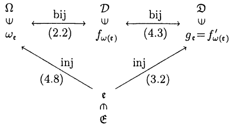
Fig. 1. The topological ends of G induce corresponding directions and graph-theoretical ends.
