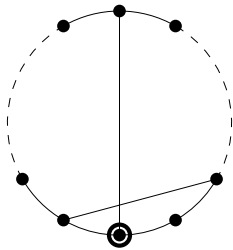
(b) Case 2 (one of the possibilities).
