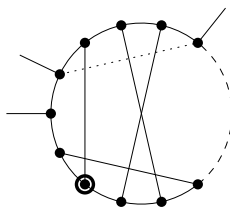
Figure 15: A deficient vertex u of type II^* .
