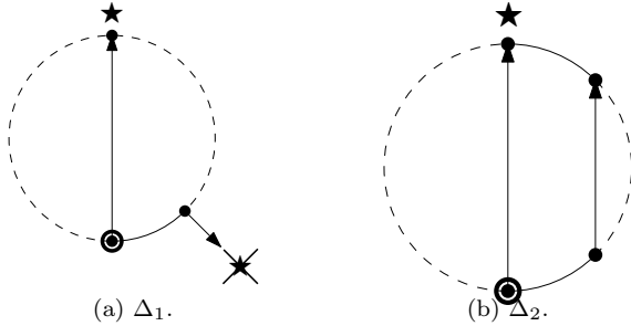
Figure 5: The symbol at u'_+ in the diagram defining the template \Delta_1 becomes removable if we add the assumption that u'_+ = v_- .
