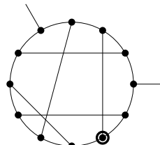
(f) Type III.
