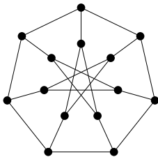
Figure 1: The generalised Petersen graph.
