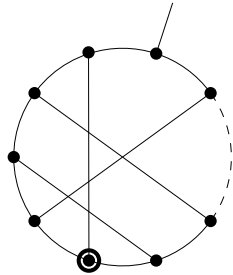
(c) v has type Ib.
