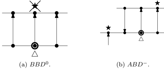
Figure 9: The events used in Case 1 of the proof of Lemma 8.
