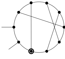
(e) v has type IIa.
