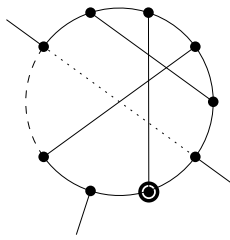
(b) Type Ia.
