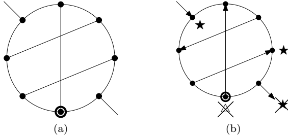
Figure 20: (a) A configuration in Subcase 2.2 of the proof of Proposition 10. (b) The event C_1C_2D^+ .
