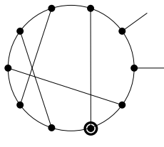
(e) Type IIa.
