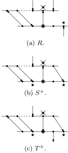
Figure 30: Events used in the proof of Proposition 13(ii) for vertices of type 0. Only the possibility that u'_{-2} = (u'_-)_- is shown, but the events remain valid if u'_{-2} = (u'_-)_+ (i.e., if the chords of Z incident with u_- and u_{-2} cross).
