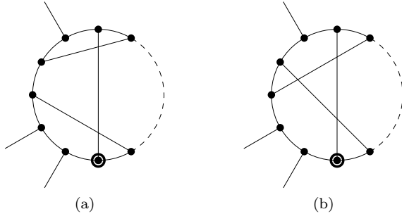
Figure 21: Two cases where the event ABD^+ cannot be used in Subcase 3.1 of the proof of Proposition 10.
