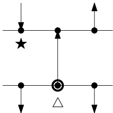
Figure 18: The event BBD^+ .
