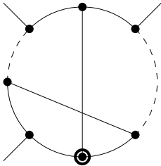
(a) v has type I.
