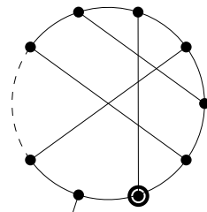
(c) Type Ib.
