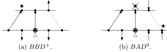
Figure 12: Some of the events used in Case 4 of the proof of Lemma 8.
