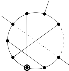
(b) v has type Ia.
