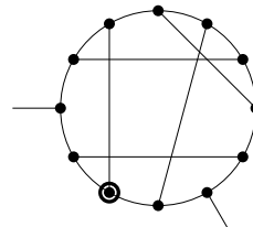
(f) v has type III.
