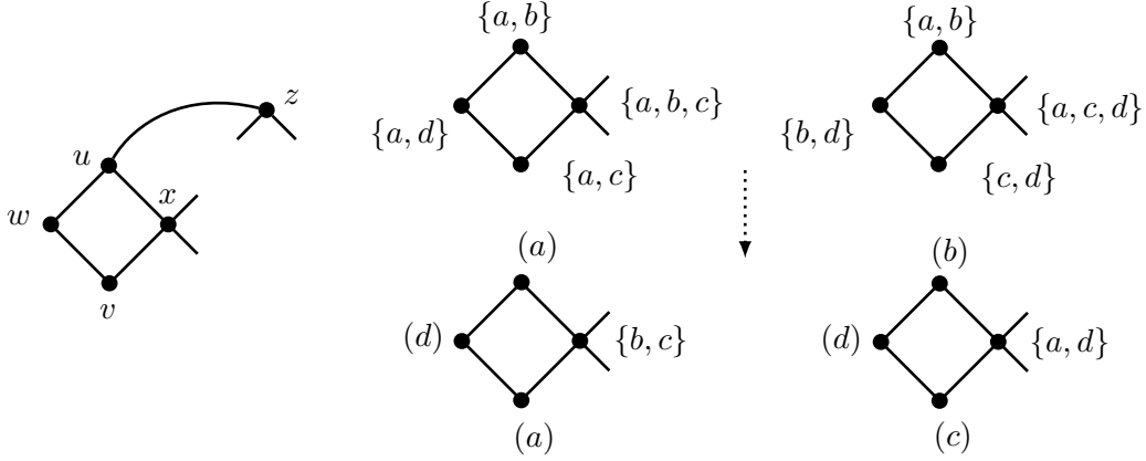
Figure 2: The 4-face in the induction step.
