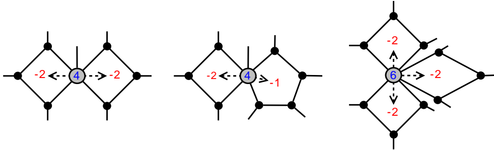
Figure 3: Illustration of Rule 1. The grey vertices have a sufficient charge to eliminate the negative charges of the incident 4-faces and 5-faces.
