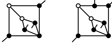
Figure 8: Two 5-faces and a 5-face with a 6-face sharing an edge and one more vertex. The 5-faces are considered proper with respect to the black vertices.
