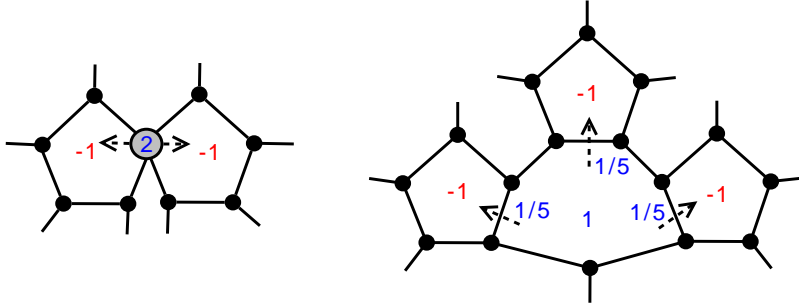
Figure 6: Illustration of Rules 4 and 5. Discharging touching 5-faces and distributing charge 1 from a 7-face to adjacent 5-faces.
