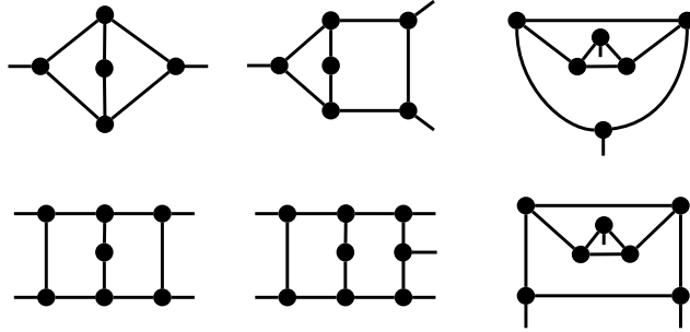
Figure 6: Illustration of Rules 4 and 5. Discharging touching 5-faces and distributing charge 1 from a 7-face to adjacent 5-faces.
