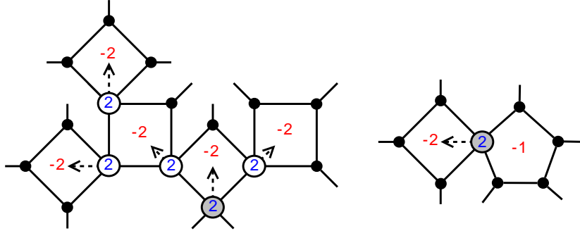
Figure 5: Illustration of Rule 3. The grey vertex eliminates the negative charge of the incident 4-face. The other white shared vertices then become non-shared. Note that the negative charge of the 5-face is not discharged.
