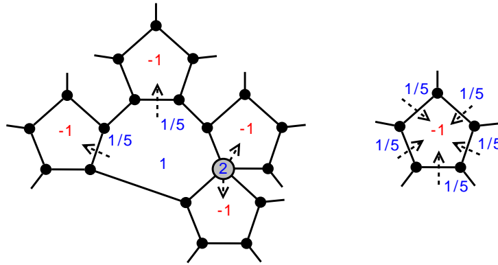
Figure 8: Two 5-faces and a 5-face with a 6-face sharing an edge and one more vertex. The 5-faces are considered proper with respect to the black vertices.
