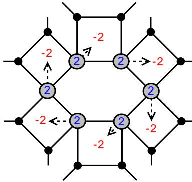
Figure 4: Illustration of Rule 2. A cycle of touching 4-faces. The arrows illustrate sending charges along the cycle.
