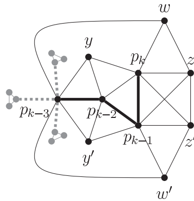
FIG. 4. Vertices w and w' and position of T .
