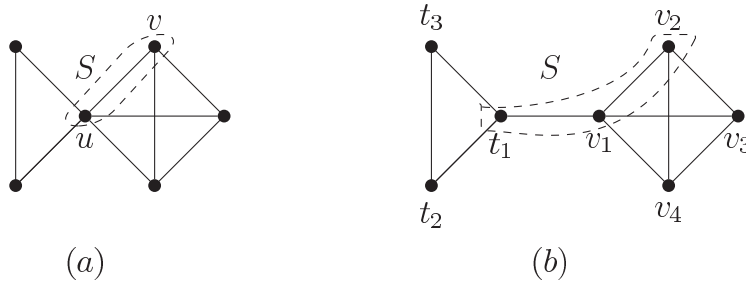
FIG. 1. The configurations of Claims 11 and 12.
