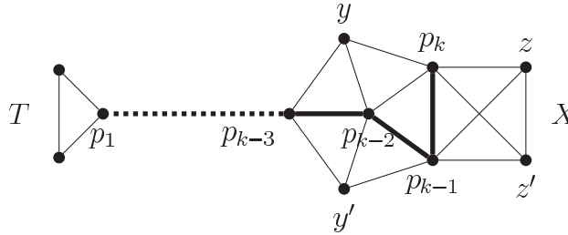
FIG. 3. Positions of T , X , y , and y' .
