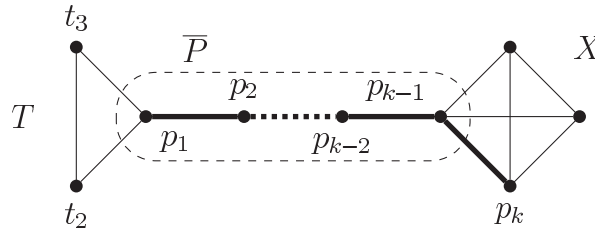
FIG. 2. Paths P and \bar{P} connecting dangerous configurations.
