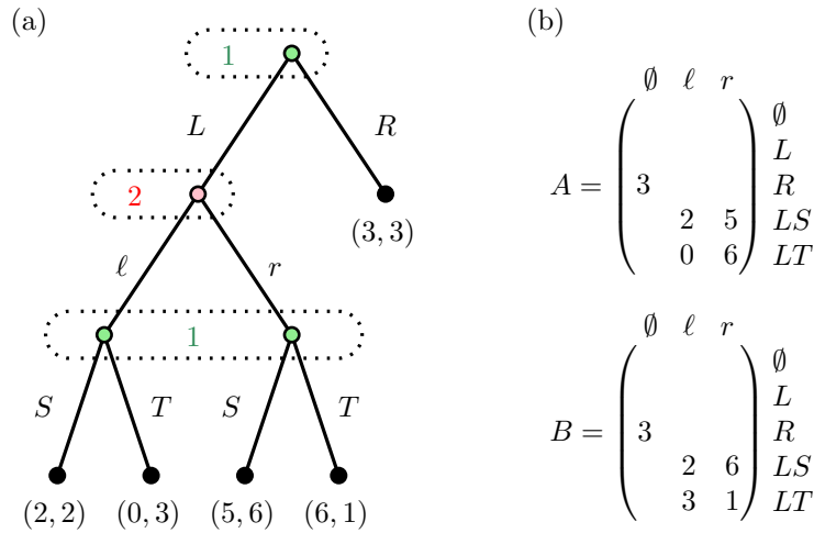
Figure 2.10: (a) An extensive game from Example 2.58. (b) Its sequence form payoff matrices.
