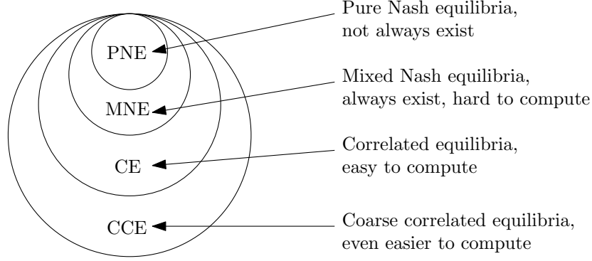
Figure 2.3: A hierarchy of variants of Nash equilibria.
