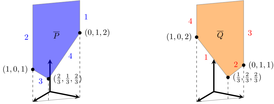
Figure 2.1: The best response polyhedra \bar{P} and \bar{Q} for the game Battle of Sexes. The labels of points in the facets are denoted by blue and red, respectively, numbers.
