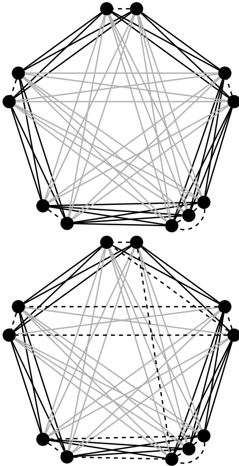
FIGURE 1. G_{ex}(11) and another element of \mathcal{G}_{11}
