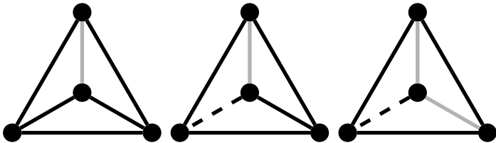
FIGURE 2. Representative elements of \mathcal{H}(2, 1, 0) , \mathcal{H}(1, 1, 1) and \mathcal{H}(0, 2, 1) .
