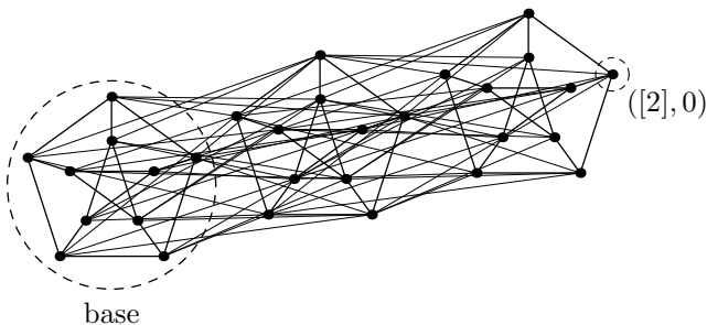
Figure 5: The ray R_{5,2,2}^{[2]} .
