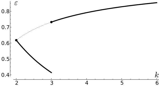
Figure 1: The values of g(k, 4) .
