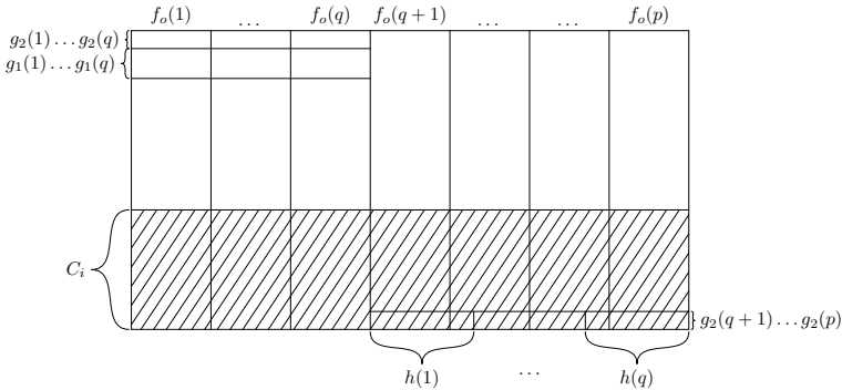
Figure 13: The construction of a fractional coloring in Theorem 6.3.
