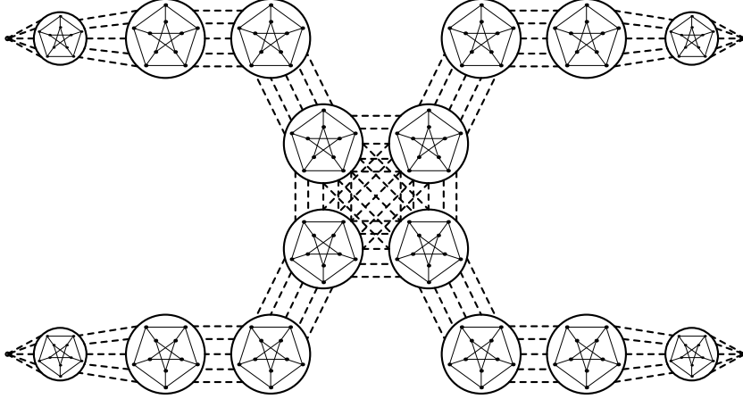
Figure 3: A sketch of the graph P_{5,2,9}^1 (some rays are omitted).
