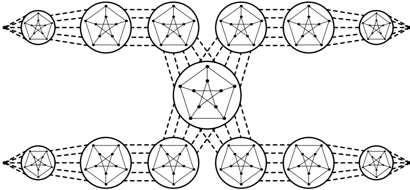
Figure 2: A sketch of the graph P_{5,2,8}^1 (some rays are omitted).
