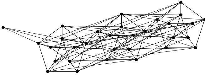
Figure 1: The ray S_{5,2,3} .
