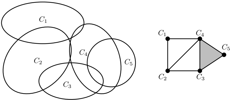
Figure 1: A 2-representable complex and its nerve.
