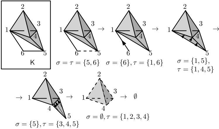
Figure 2: A 2-collapsing of a simplicial complex.
