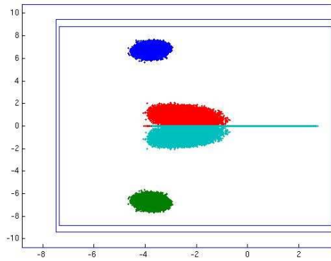
Figure 4: Eigenvalue set and enclosures to Example 4.
