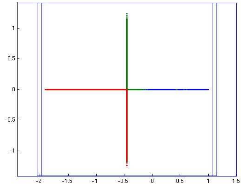
Figure 3: Eigenvalue set and enclosures to Example 3.
