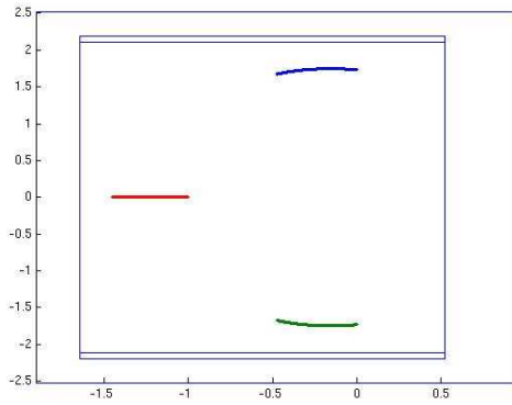
Figure 2: Eigenvalue set and enclosures to Example 2.
