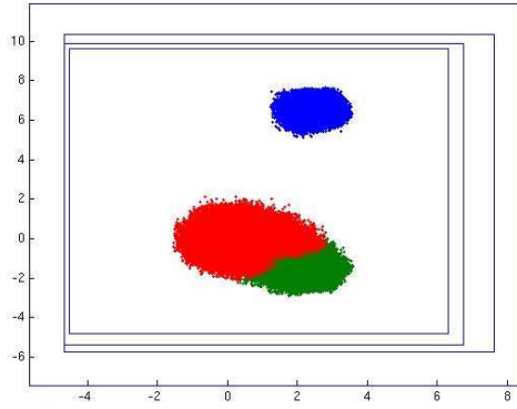
Figure 1: Eigenvalue set and enclosures to Example 1.
