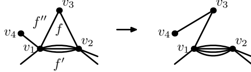
Figure 1: Notation used in the proof of Lemma 12 and the swap.
