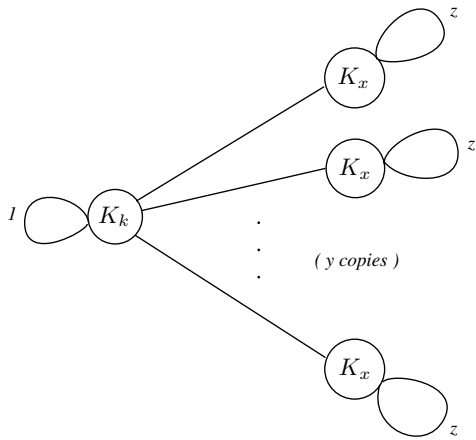
Figure 6: The graph H_{k,x,y,z} . This can be viewed as an ornamented star K_{1,y} : the central vertex is replaced by k twin vertices forming a clique with loops on each vertex, all edges having weight 1. The y pendant vertices are replaced by x -cliques, with loops of weight z attached to each vertex. The single lines joining cliques each stand for kx edges joining all pairs of vertices between K_k^1 and K_x^z . All edges are weight 1 unless otherwise indicated. The case z = 1 is the graph of [12, Figure 6], for which \text{hom}(G, H_{k,x,y,1}) = k^{|V(G)|} Q(G; x/k, y) . The case y = 1 gives –after renaming parameters– the graph in Figure 7.
