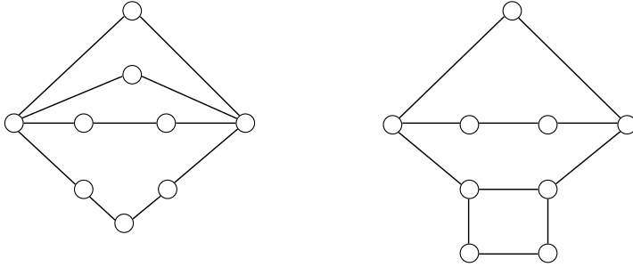
Figure 4: Graphs with the same chromatic polynomial but different 2-state Potts partition functions
