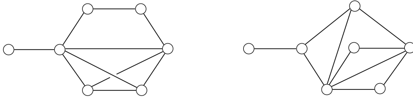
Figure 3: Graphs with different chromatic number and different clique number but the same 2-state Potts partition function.
