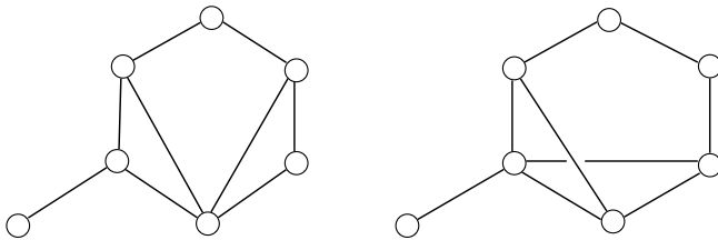
Figure 2: Simple graphs with the same 2-state Potts partition function but different Tutte polynomials. They also have different chromatic polynomials.
