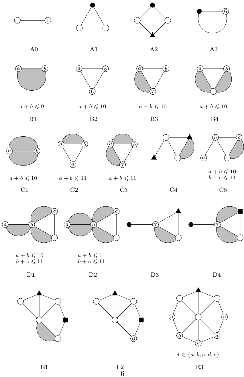
Figure 1: The reducible configurations.
