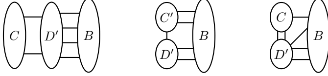
Figure 7: Smaller cyclic edge-cuts of G in the proof of Lemma 22.
