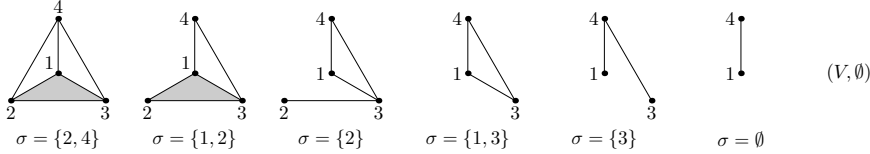
Figure 1: An example of 2-collapsing.
