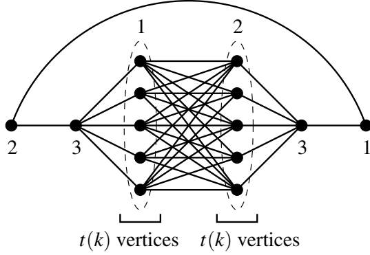
Figure 2: The graph H_k .
