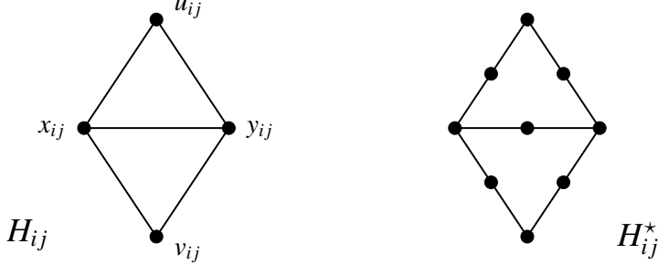
Figure 1: The graphs H_{ij} and H_{ij}^* .
