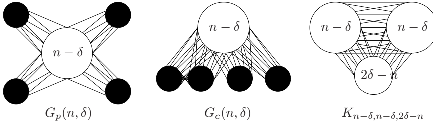
Figure 2: The extremal graphs, for the special case r_p(n, \delta) = r_c(n, \delta) = 4 .
