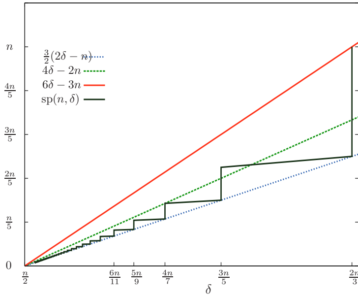
Figure 1: The behaviour of \text{sp}(n, \delta) .
