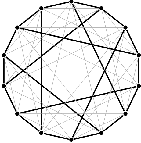
Figure 1: A special admissible colouring of K_{14} by 23 colours. Thick edges are those of L_2 (hence each of them has a colour of its own, say from \{2, \dots, 22\} ), missing edges represent colour 0, grey edges represent colour 1.
