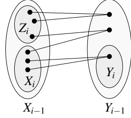
Figure 2: X_i = X_{i-1} \setminus Z_i and Y_i = Y_{i-1}^{X_i} .
