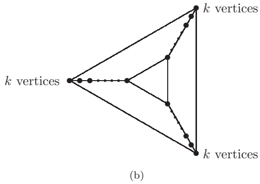
Figure 1: (a) A planar graph G with maximum degree \Delta = 2k and \omega(G^2) = \chi(G^2) = 3k + 1 = \lfloor \frac{3}{2} \Delta \rfloor + 1 . (b) A planar graph H with maximum face degree \Delta^* = 2k and \chi^*(H) = 3k = \lfloor \frac{3}{2} \Delta^* \rfloor (see Subsection 1.2 below).
