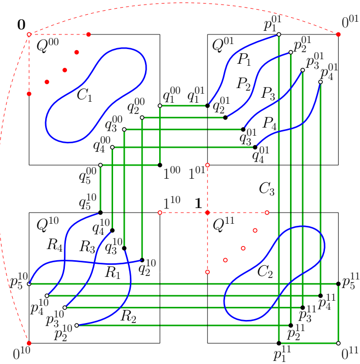
Figure 10: The construction in Theorem 1 with n = 7 .
