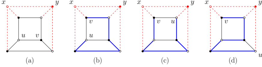
Figure 1: All configurations (up to isomorphism) in Proposition 2 for n = 3 .
