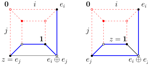
Figure 2: The Hamiltonian paths in Proposition 3 for n = 3 .
