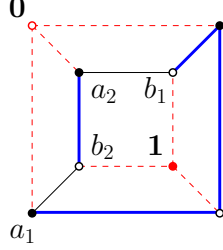
Figure 5: The only (up to isomorphism) configuration in Lemma 1 for n = 3 .
