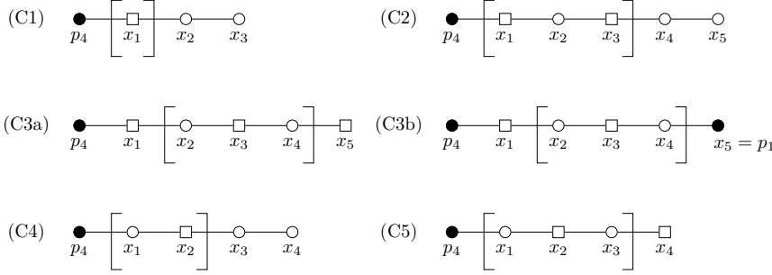
Figure 5: The construction of the set X_1
