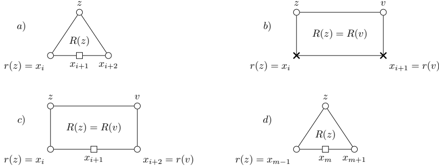
Figure 6: The construction of the set X_2
