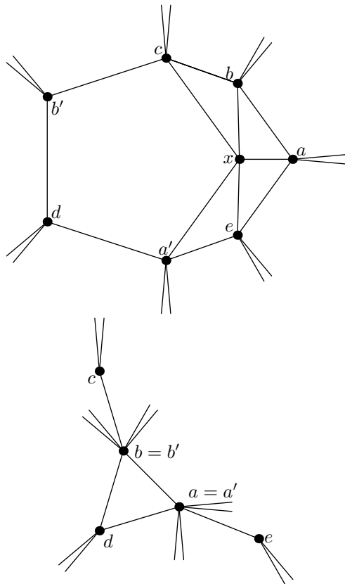
Figure 3: A 5-face incident with two consecutive 5-vertices and its reduction.
