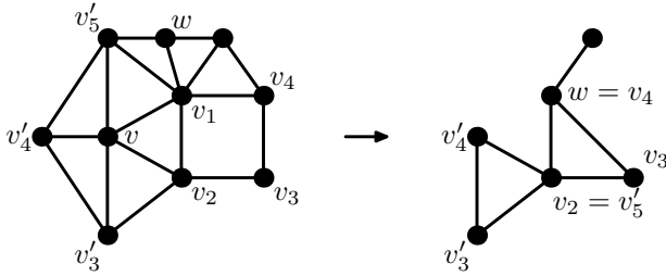
Figure 5: A reduction of a 4-face with a vertex of degree five adjacent to a close pentagonal vertex.
