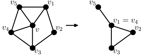
Figure 2: A vertex of degree four with five cyclic neighbors and its reduction.
