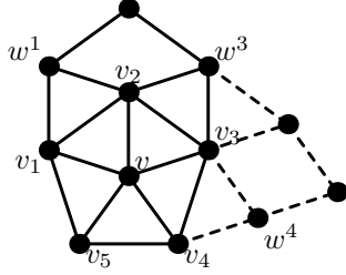
Figure 10: Notation used in the proof of Lemma 15.
