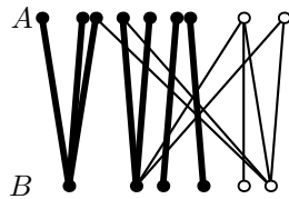
Figure 2: An up-forest
