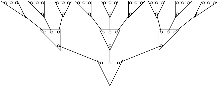
Figure 1: Graph T_{3,2}(G) from the proof of Lemma 2.2.
