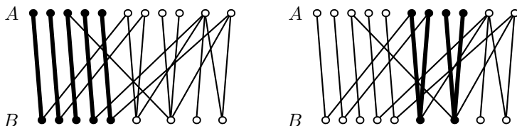
Figure 3: An illustration of Lemma 3.1
