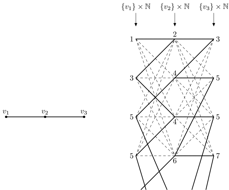
Figure 1: The path P_3 and the pair (R_{P_3}, T_{P_3}) . Labels at vertices are the smallest such i that the corresponding vertex belongs to T_{P_3}^i . For example T_{P_3}^3 consist of vertices with labels 1, 2 and 3, and thick edges connecting them.
