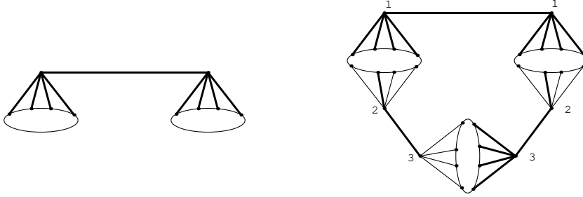
Figure 1: Graphs R and G
