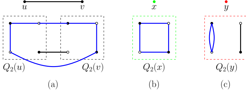
Figure 7: The 2-factor C of Q_{n+2} - V(M) .
