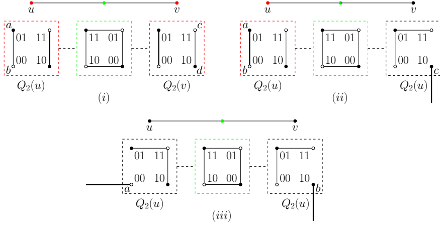
Figure 6: An illustration for Lemma 4.
