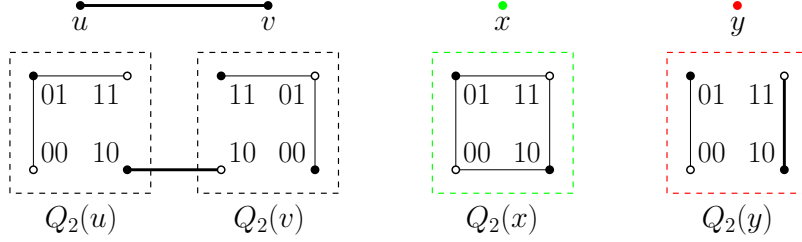
Figure 5: S(u) = S(v) = \{\{00, 01\}, \{01, 11\}\} , S(x) = E(Q_2) , S(y) = \{\{00, 01\}\} .
