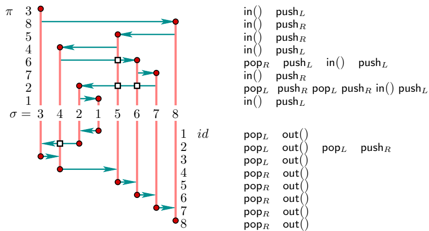
Figure 2: Sorting the input permutation \pi = 38546721 via \sigma = 34215678 . Time corresponds to the vertical axis, movements of the head are horizontal arrows. The four extra moves where an element has to switch between stacks are indicated by squares. On the right we give the sequence of stack operations for sorting \pi via \sigma .
