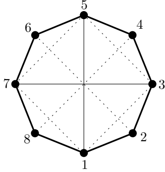
Figure 2: The octagon example.
