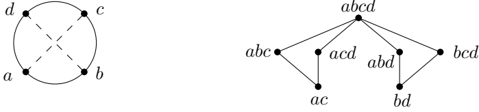
Figure 1: The square example (left) and its top poset (right).
