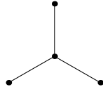
Figure 2: A complex that is 1-collapsible but not 1-representable.
