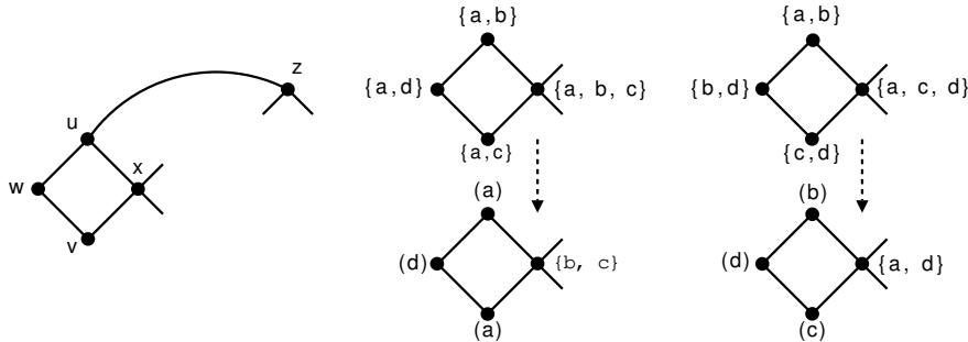
Figure 2: The 4-face in the induction step.
