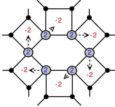
Figure 4: Rule 2. A cycle of 4-cycles and moving charges along the cycle.
