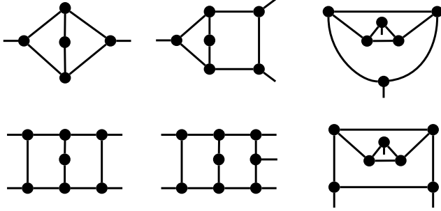
Figure 7: Two small cycles drawn as a faces that share two edges require a vertex of degree two or triangles.
