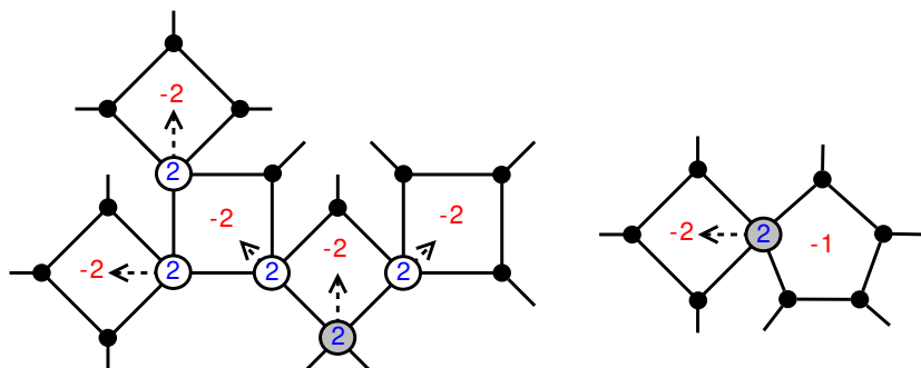
Figure 5: Rule 3. The grey vertex eliminate the negative charge of the adjacent 4-face. The other white shared vertices then become non-shared. Note that the negative charge of the 5-face is not discharged.
