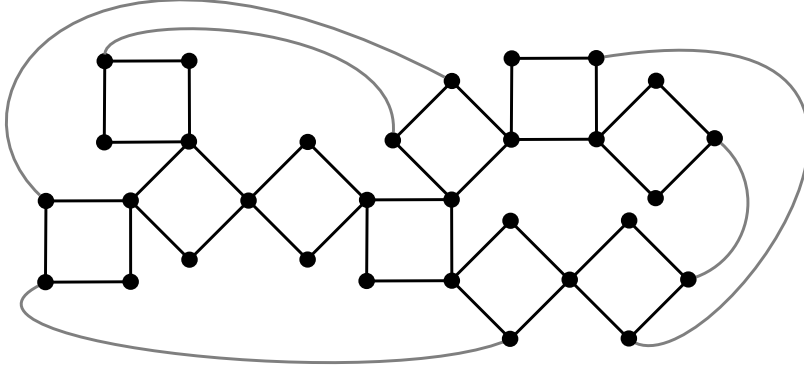
Figure 1: C_4 -arbor
