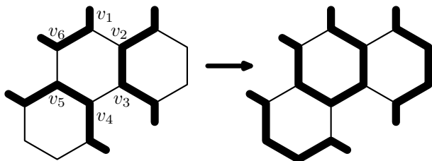
Figure 10: The configuration analyzed in the proof of Lemma 9.
