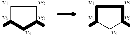
Figure 2: Prolonging the cycle C if the graph G contains a white face of size five.
