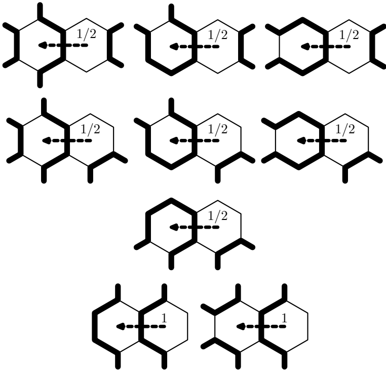
Figure 3: Configurations (up to symmetry) to which Rules A and B are applied.
