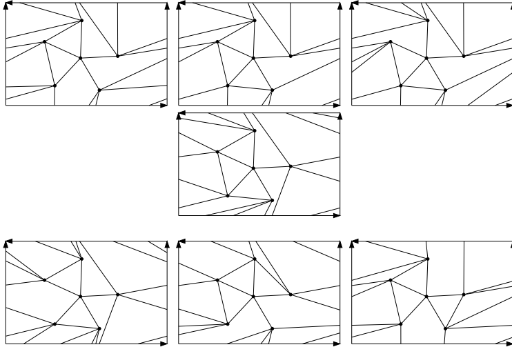
Figure 3: The list of all seven non-isomorphic 2-cell embeddings of K_6 on the Klein bottle.
