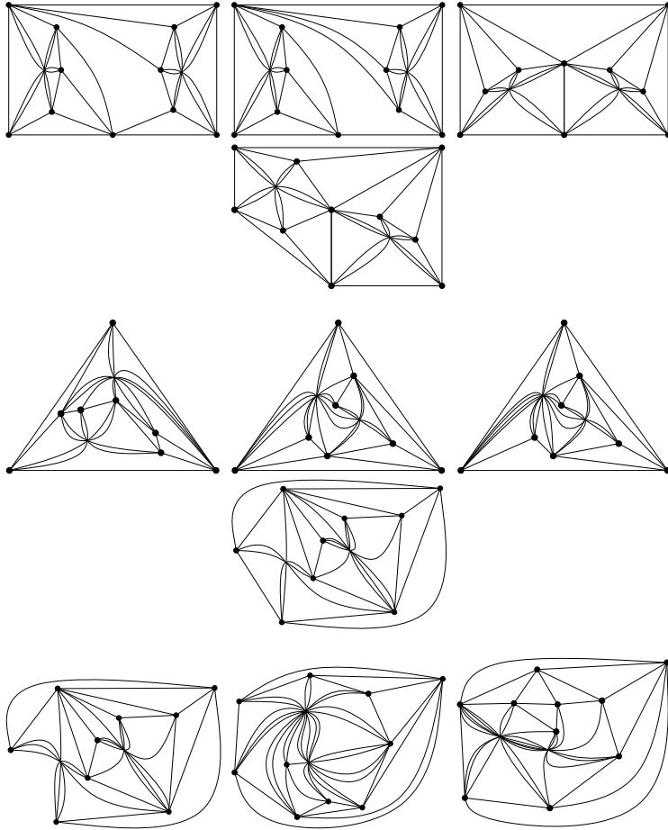
Figure 4: The list of 11 non-isomorphic embeddings of 6-critical graphs on the Klein bottle that are distinct from K_6 . The graphs are drawn in the plane with two cross-caps.
