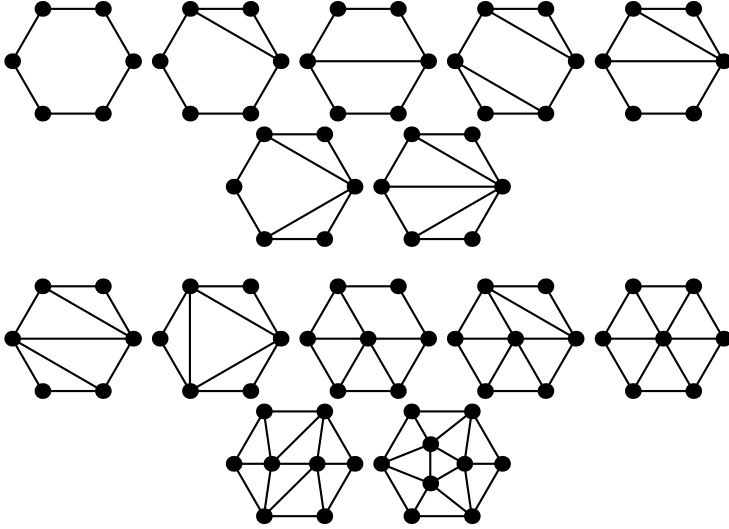
Figure 1: The list of all 6-minimal graphs.
