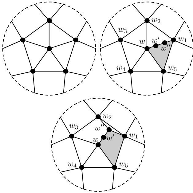
Figure 5: The unique embedding of K_6 in the projective plane and its two possible expansions.
