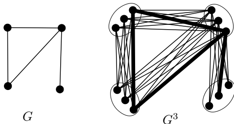
Figure 1: Example of inflating the graph G by factor 3.
