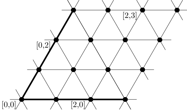
Figure 2: The infinite triangular lattice \Gamma_\Delta with an origin and two axes.
