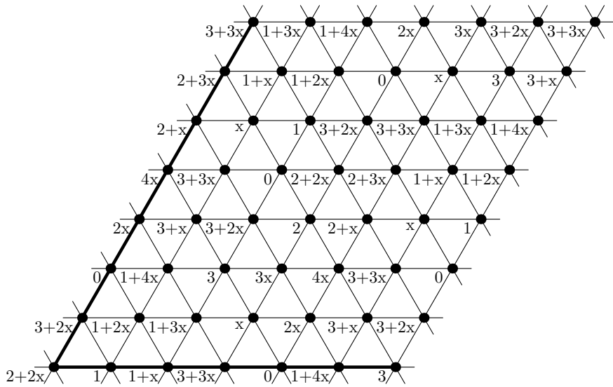
Figure 3: A part of the labelling of the infinite triangular lattice.
