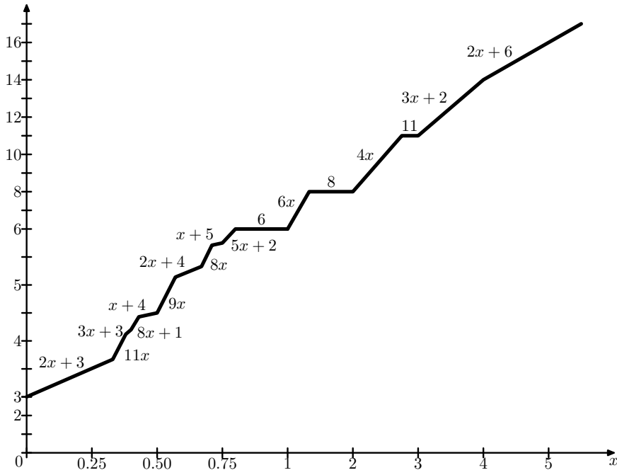
Figure 1: The optimal value of \lambda(\Gamma_\Delta; x, 1) . Note that some parts of the graph are enlarged to reflect the behavior \lambda(\Gamma_\Delta; x, 1) in more detail.
