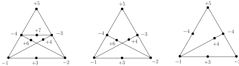
Figure 8: A_i -configuration in I_{i+2}
