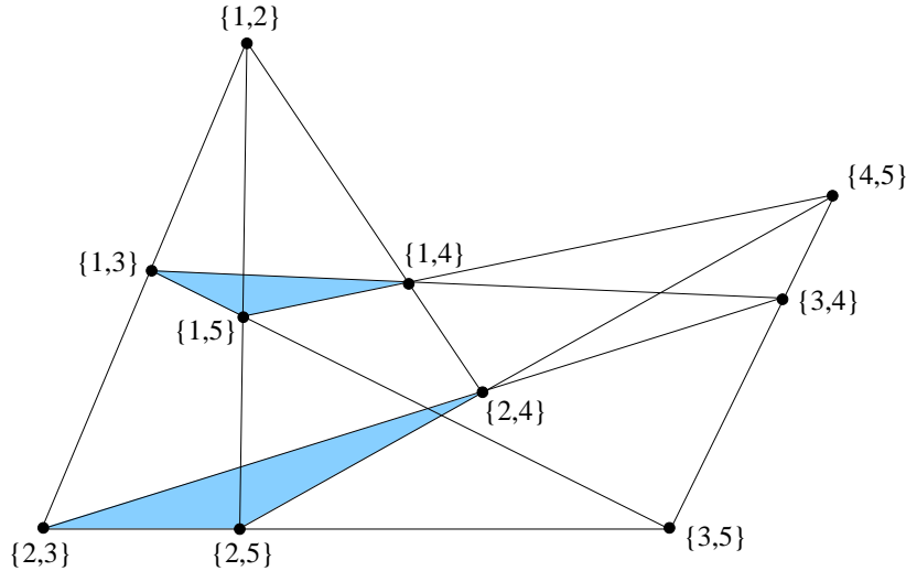
Figure 9: Desargues configuration
