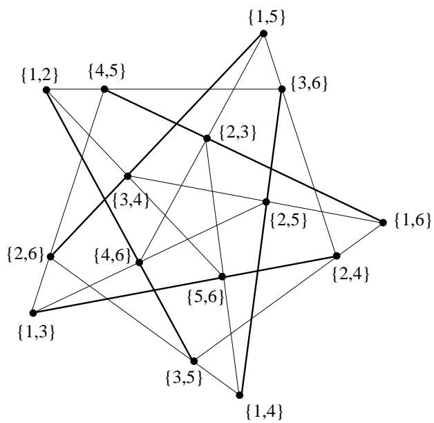
Figure 10: Cremona-Richmond configuration
