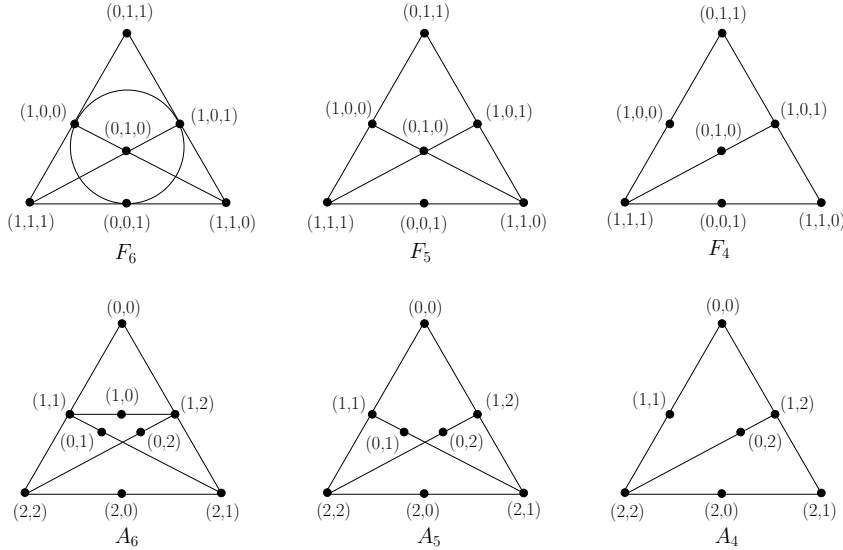
Figure 4: Projective and affine configurations in Theorem 3.2
