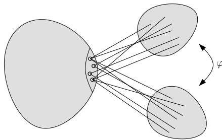
FIGURE 4. \varphi is an involutive automorphism exchanging two connected P_k -free subgraphs.
