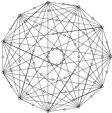
FIGURE 1. The subdivision graph S(K_n) of K_n . Every edge of the maximum induced matching is incident to a principal vertex hence \beta^*(S(K_n)) = n .
