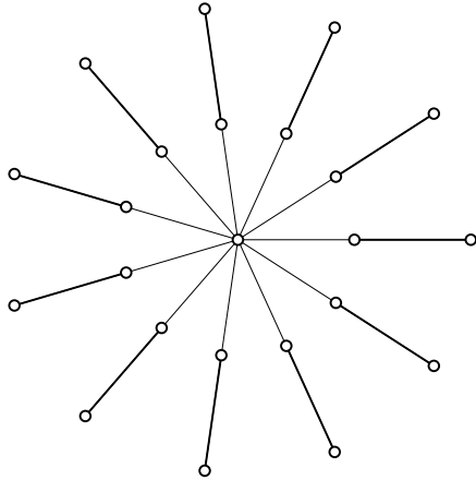
FIGURE 2. The subdivision graph S(S_n) of the star S_n . An induced matching of size n is easily found but these graphs, although having no clones and bounded \nabla_i for all i \geq 0 , have no two disjoint induced P_3 .
