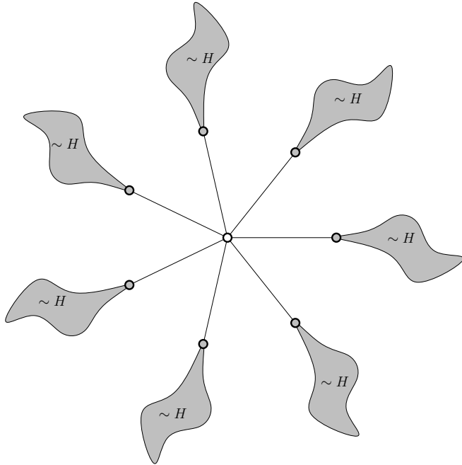
FIGURE 3. From a connected graph H with diameter k - 1 , one can build a class with bounded expansion so that each graph in the class contains an induced P_k but not two disjoint ones.
