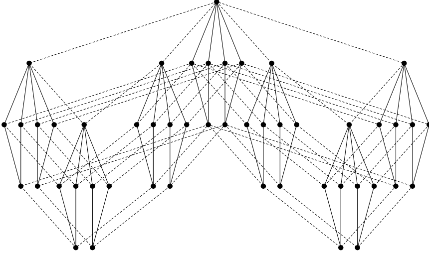
Figure 3: The poset \mathcal{P}_{w(H)} for m = 2 .
