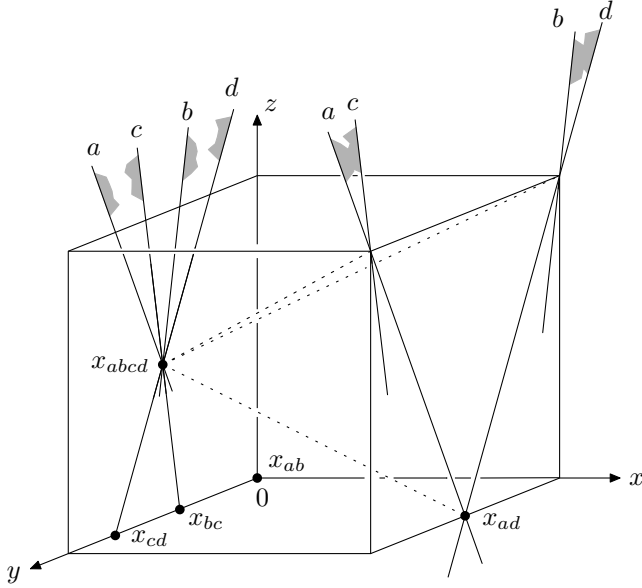
Figure 5: A linear program in \mathbf{R}^3 essentially representing the square example.
