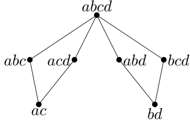
Figure 2: The poset \mathcal{P}_{w_0(H_0)} for the square example.
