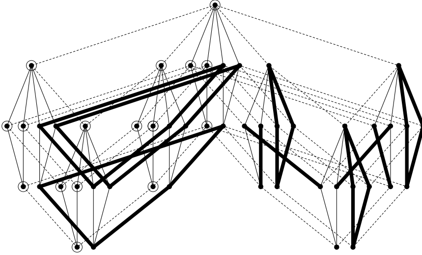
Figure 4: A covering of \mathcal{P}_{w(H)} by disjoint cubes; a 4-dimensional cube is marked by circles around its vertices.
