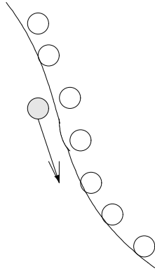
Figure 3: Idem0=particles movement in Euclid space. idem1=particles movement in field along geodesic. idem2 = multiparticle simulating action of the field. Considered as quantum particle, i.e., one-particle, it comprises abstraction of the action of the field.
