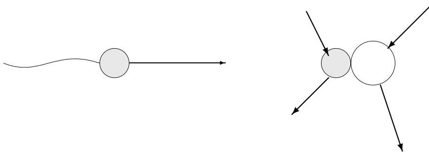
Figure 1: Left: First state: Particle in free motion = particula in se state. Right: Second state: Particula collidens state = particle in 5D manifold: locally in a point of Euclid space with pair of vectors attached, showing the directions where the second particle in collision came from and went to, in R^3 \cdot V^2 . Adding the aspect of thinking to the self-reference system, we would like to speak of the state particula in se meditans , or even particula in se cogitans ergo existens [7, 6].
