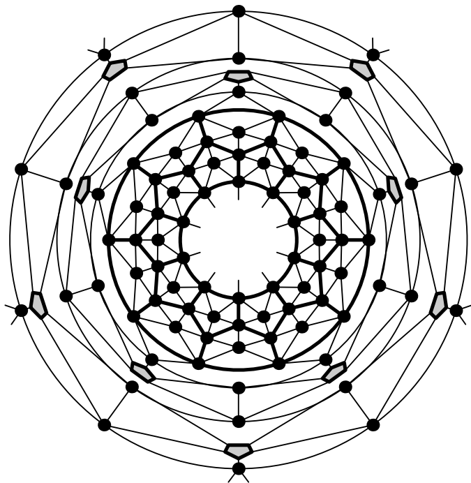
Figure 7: Edges joining an A -gadget and a B -gadget.
