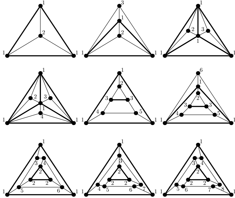
Figure 2: 3-connected plane graphs G with n vertices, n = 4, \dots, 12 , that have non-rainbow colorings with \lfloor \frac{7n-8}{9} \rfloor colors. The edges of G that are monochromatic in such a coloring are drawn bold. The colors assigned to the vertices are represented by numbers.
