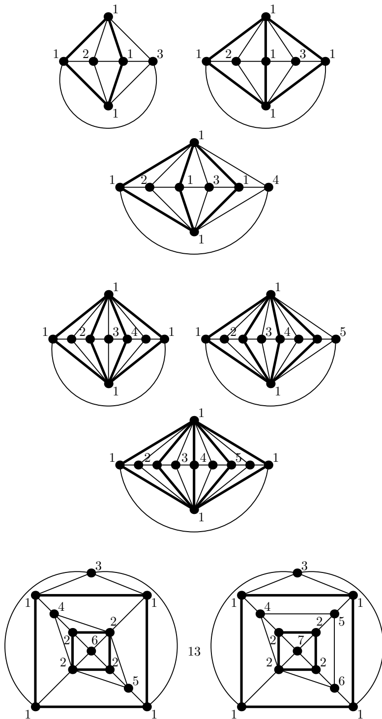
Figure 4: 4-connected plane graphs G with n vertices, n = 6, 7, \dots, 13 , that have non-rainbow colorings with \lfloor \frac{5n-6}{8} \rfloor colors if n \neq 11 , i.e., n \not\equiv 3 \pmod{8} , and with \lfloor \frac{5n}{8} \rfloor - 1 = 5 colors, if n = 11 . The edges of G that are monochromatic in such a coloring are drawn bold. The colors assigned to the vertices are represented by numbers (some vertices are not labeled with numbers; those vertices are colored with 1).
