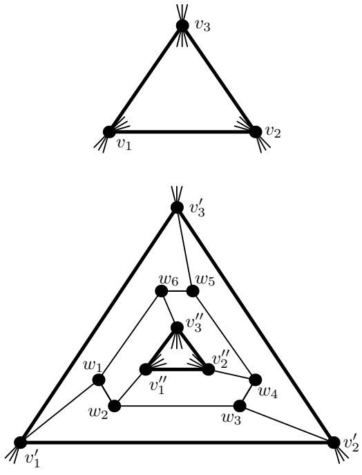
Figure 1: A construction presented in Lemma 4. The monochromatic edges in the configurations are drawn bold.
