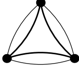
Figure 2: The bigraph K_3^2 .
