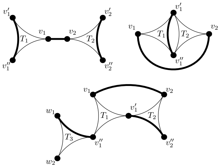
Figure 9: The configurations in the case \alpha = 0, \beta = 1 and the vertices of the pair are not contained together in any of the triples.
