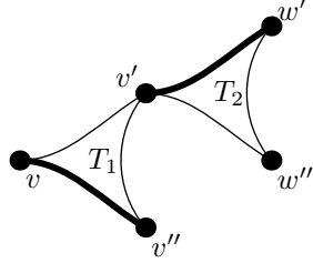
Figure 11: The configuration considered in the case \alpha = 1 and \beta = 0 .
