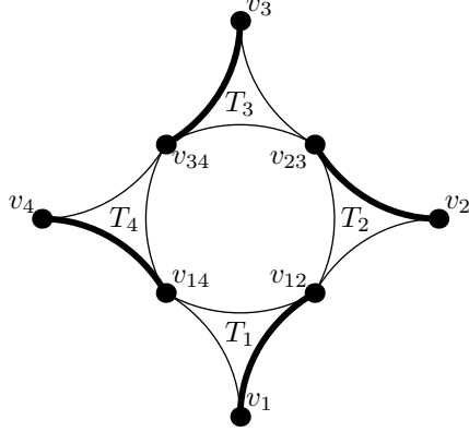
Figure 4: The configuration in the case that \alpha = 0 , \beta = 0 , there are no two triples sharing two vertices, there are no three triples such that any two of them share a vertex, and there are four triples (cyclically ordered) such that pairs of consecutive triples share a vertex.
