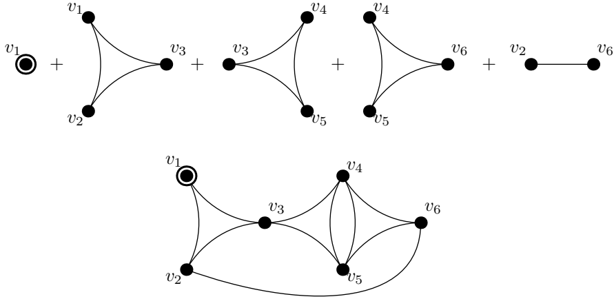
Figure 1: An example of a bigraph. The bigraph is formed by one singleton, one pair and three triples.
