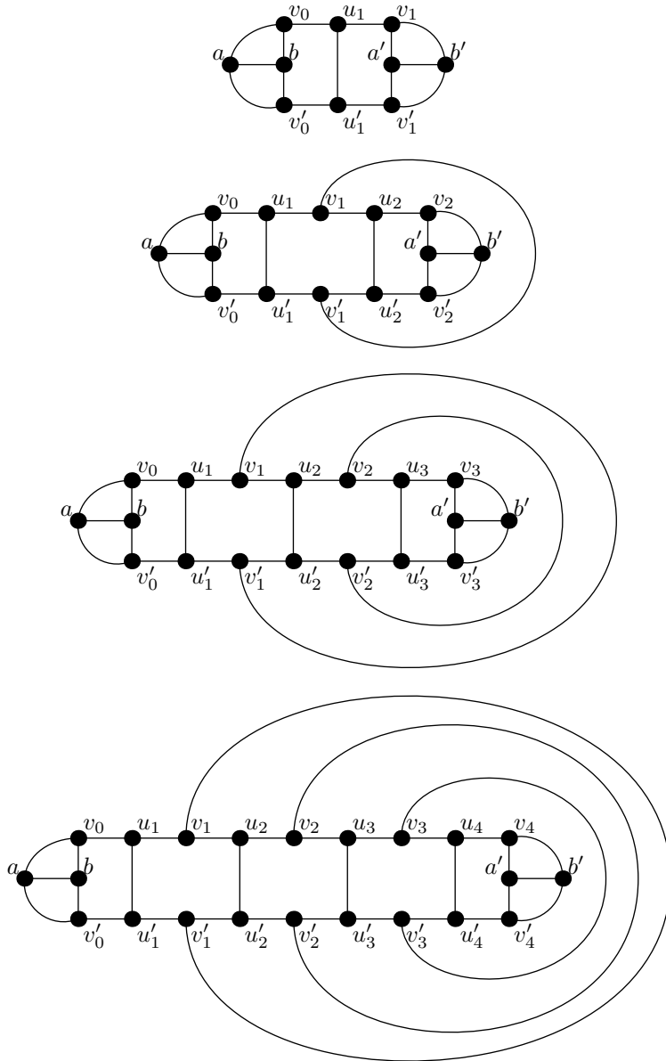
Figure 12: The graphs G_1 , G_2 , G_3 and G_4 .
