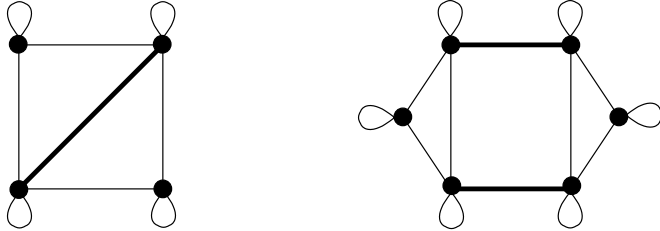
Fig. 1. Trigraphs for some partition problem relevant for perfect graphs.
