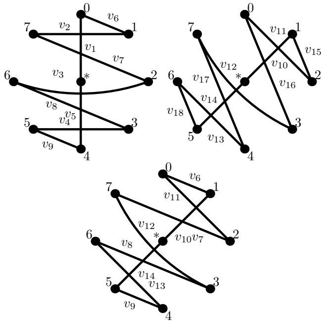
Figure 2: The edges corresponding to the vertices v_1, \dots, v_9 contained in the block B_1 and the vertices v_{10}, \dots, v_{18} contained in the block B_2 of the order of the vertices of K(9, 2) constructed in the proof of Lemma 1 (the left and the middle part of the figure). In the right part of the figure, there is depicted the subgraph formed by the last four edges of the first block and the first five edges of the second block.
