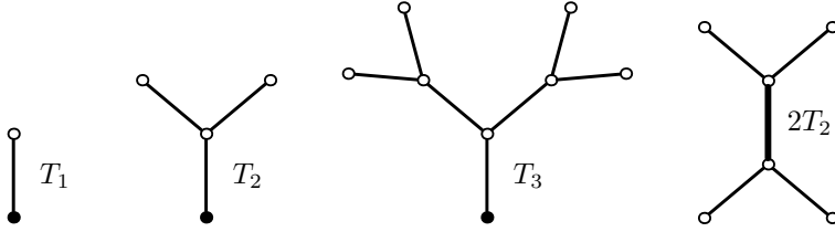
Figure 2: Illustration of definitions, root vertex/central edge are emphasized.
