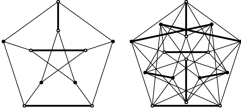
Figure 1: Petersen and Clebsch graph with one cut complement emphasized, the respective bipartition of the vertex set is depicted, too. The other four cut complements are obtained by a rotation.
