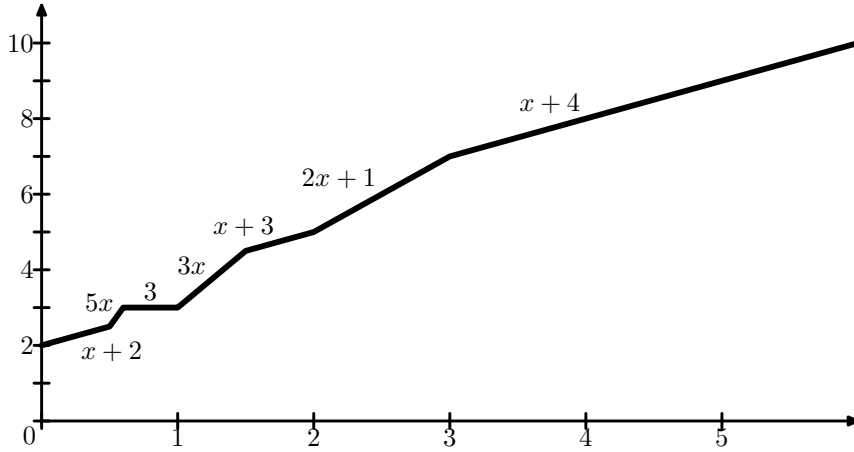
Figure 2: The function \lambda(T_3; x, 1) .
