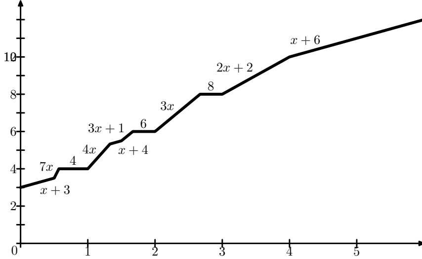
Figure 5: The function \lambda(\Gamma_{\square}; x, 1) .
