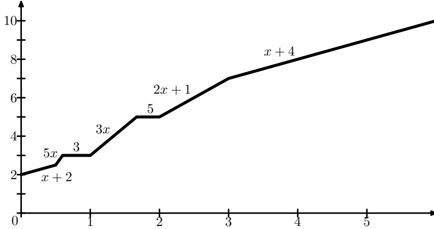
Figure 6: The function \lambda(\Gamma_H; x, 1) .
