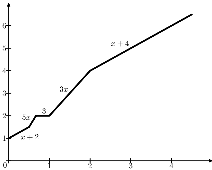
Figure 1: The function \lambda(P_n; x, 1) for paths P_n with at least seven vertices ( n \geq 7 ).
