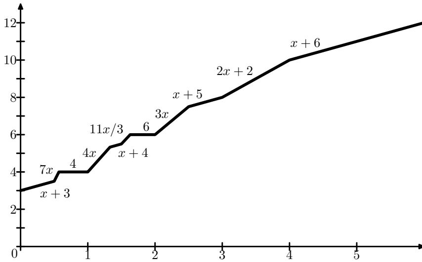
Figure 3: The function \lambda(T_4; x, 1) .
