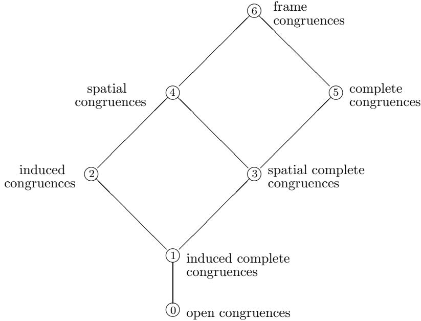
Diagram: congruences on a spatial frame L = \mathfrak{D}(X)
