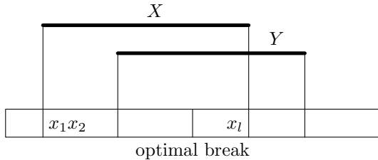
Figure 1: Illustration of Lemma 3.2
