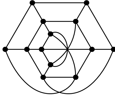
Figure 9: An example of a non-3-colorable near-quadrangulation of the Klein bottle.
