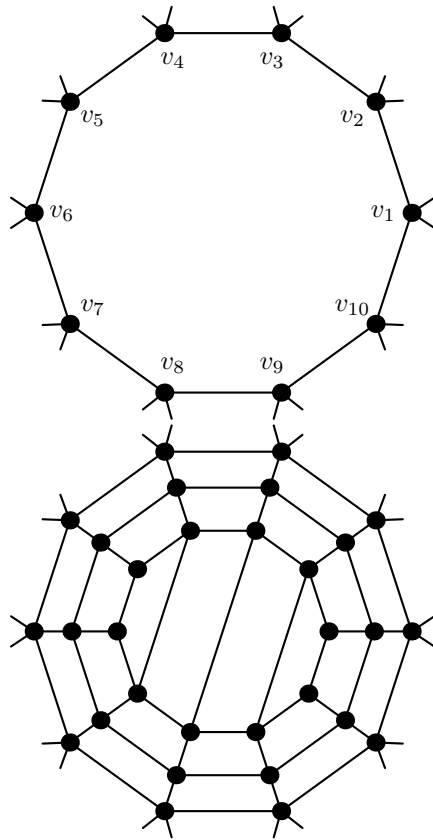
Figure 8: Replacement of the interior a face of length 10 in the proof of Theorem 2.
