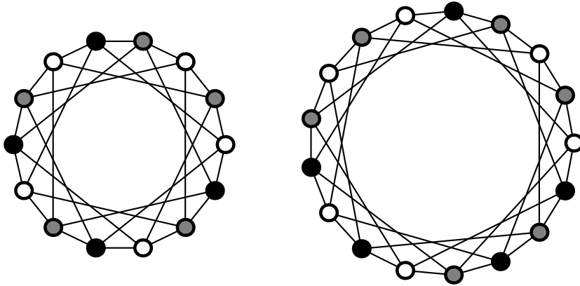
Figure 6: The graphs of the drawings Q_{14,4,1} and Q_{17,4,1} and their 3-colorings.
