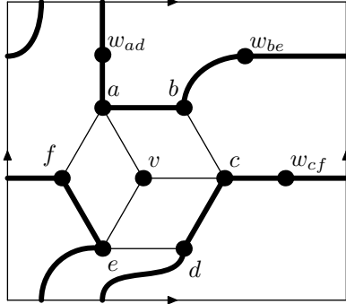
Figure 2: The unique embedding of the subgraph of G formed by the vertices v, a, b, c, d, e, f, w_{ad}, w_{be} and w_{cf} on the torus and the contractible 9-cycle aw_{ad}dcw_{cf}fe w_{be}b (drawn bold).
