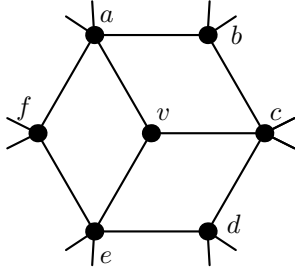
Figure 1: The notation used in the proof of Lemma 11.
