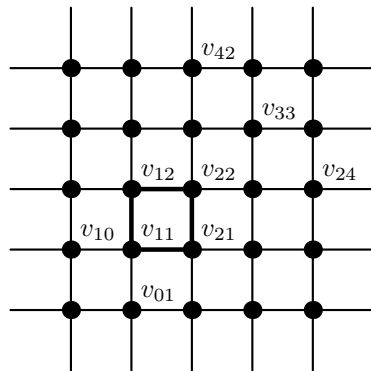
Figure 3: \mathbb{Z}^2/L for the lattice L generated by (4, 0) and (-1, 3) with one of the sets of identified vertices marked. The corresponding graph Q_{4,3,1} and its embedding on the torus is depicted in the right part of the figure.
